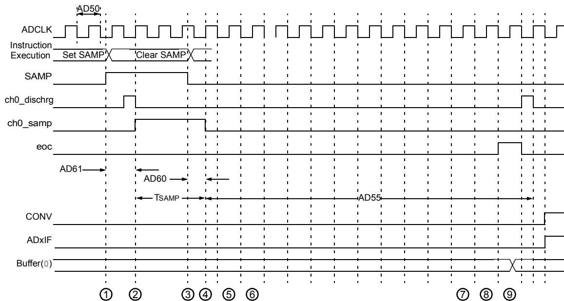
FIGURE 23-18: ADC CONVERSION (12-BIT MODE) TIMING CHARACTERISTICS (ASAM = 0, SSRC<2:0> = 000)
