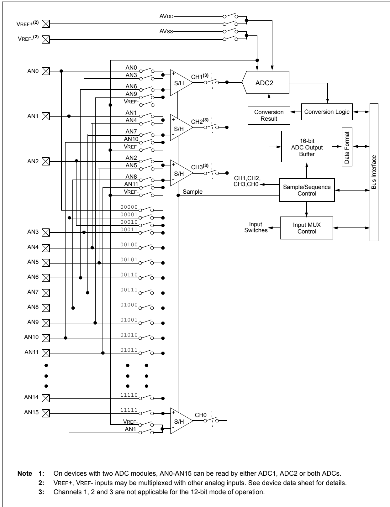
FIGURE 19-2: ADC2 MODULE BLOCK DIAGRAM (1)
