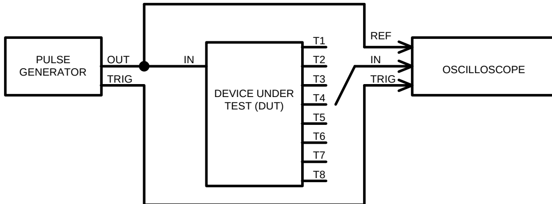
Test Setup
