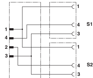
Contact assignment of M12 plugs / M8 sockets
