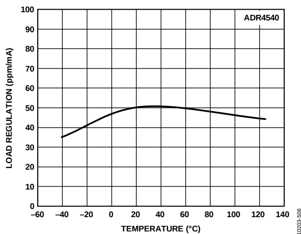
Figure 69. ADR4540 Load Regulation vs. Temperature (Sinking)
