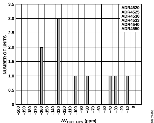
Figure 4. ADR4520 Thermally Induced Output Voltage Hysteresis Distribution
