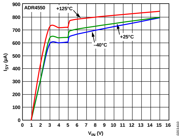
Figure 86. ADR4550 Supply Current vs. Supply Voltage
