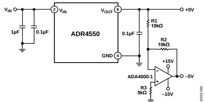
Figure 95. ADR4550 Bipolar Output Reference
