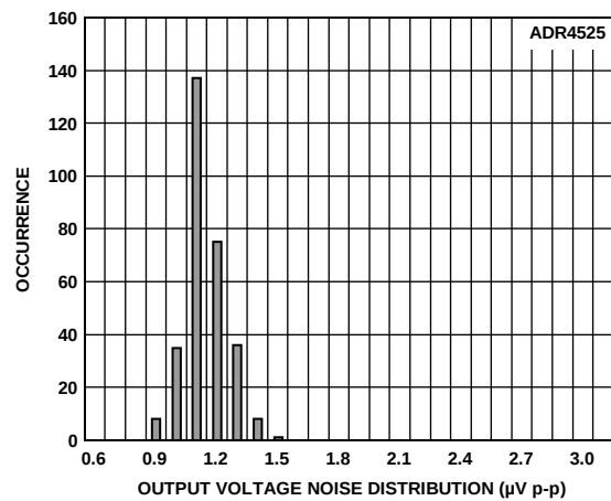
Figure 26. ADR4525 Output Voltage Noise (Maximum Amplitude from 0.1 Hz to 10 Hz)
