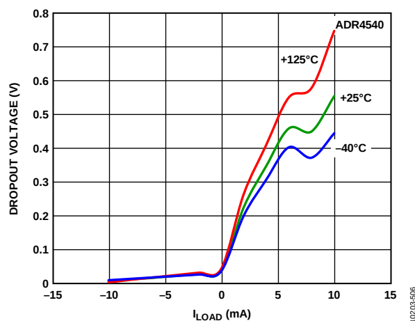
Figure 67. ADR4540 Dropout Voltage vs. Load Current
