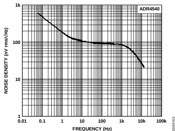
Figure 73. ADR4540 Output Noise Spectral Density
