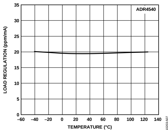
Figure 68. ADR4540 Load Regulation vs. Temperature (Sourcing)
