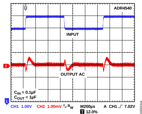
Figure 75. ADR4540 Line Transient Response
