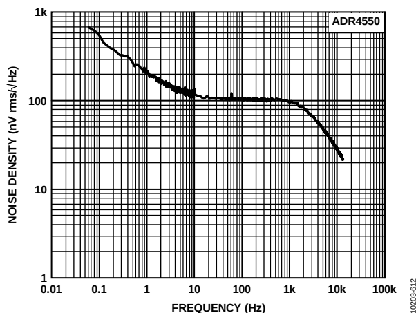
Figure 88. ADR4550 Output Noise Spectral Density
