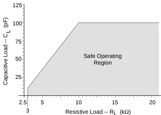
Figure 18. Maximum Loading
