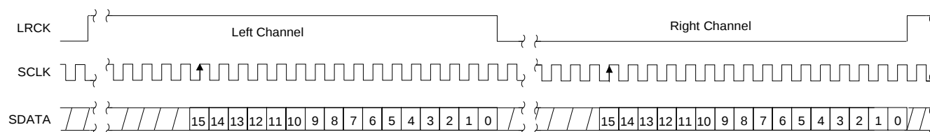
Figure 24. CS43L41 Format 4
