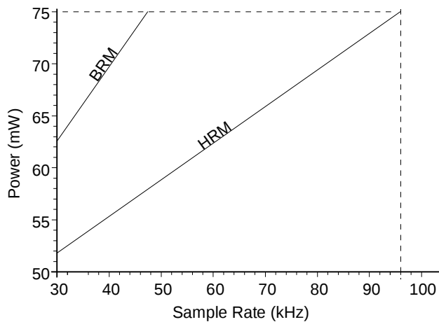
Figure 19. Power vs. Sample Rate ( V_A = 5V )
