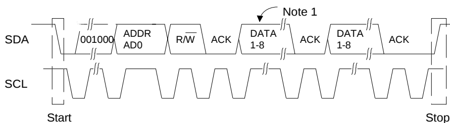
Figure 8. I²C Mode Control Port Formatting
