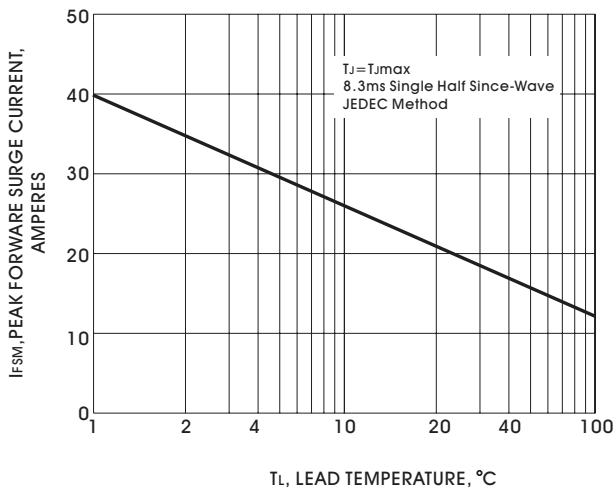
FIG. 5-MAXIMUM NON-REPETITIVE PEAK FOWARD SURGE CURRENT
