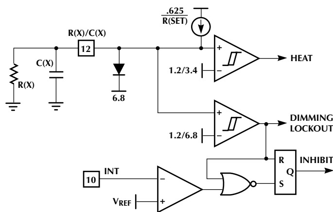
Figure 4. Lamp Preheat and Interrupt Timers
