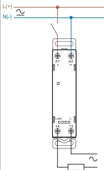
Single-phase connection (77.11)
