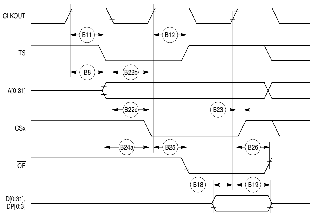
Figure 14. External Bus Read Timing (GPCM Controlled—TRLX = 0 or 1, ACS = 11)
