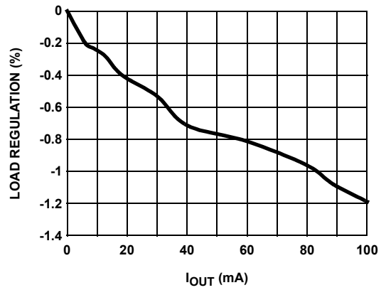
FIGURE 10. V_{\text{OFF}} LOAD REGULATION
