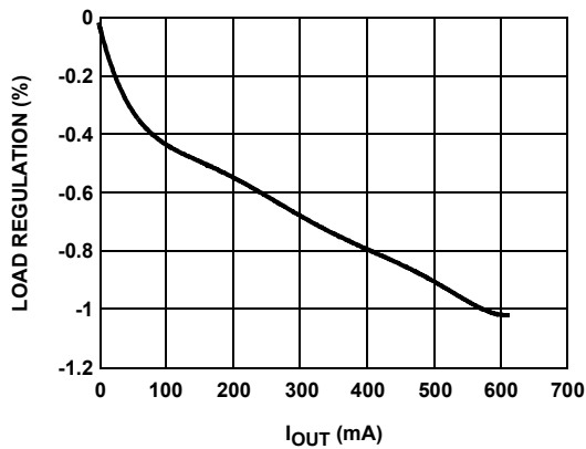
FIGURE 11. V_{\text{LOGIC}} LOAD REGULATION
