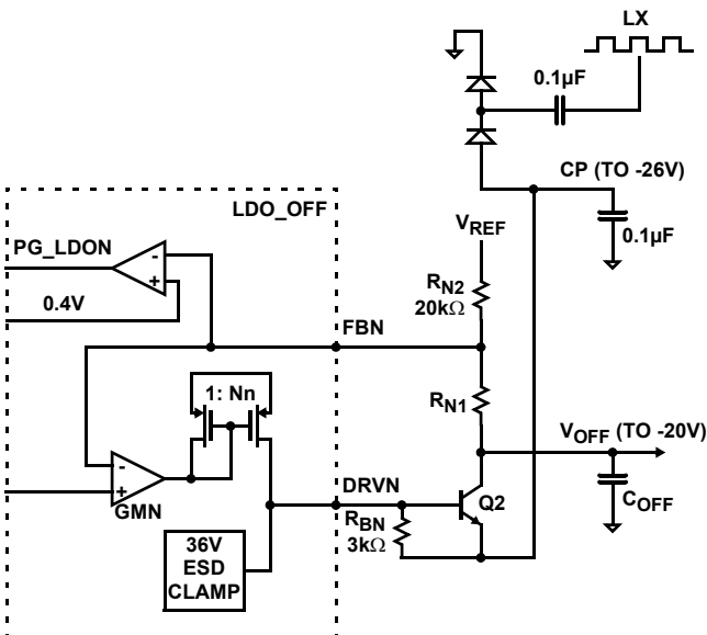
FIGURE 22. V_{\text{OFF}} FUNCTIONAL BLOCK DIAGRAM
