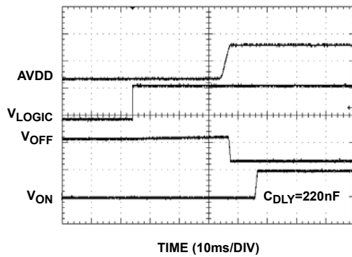
FIGURE 15. START-UP SEQUENCE
