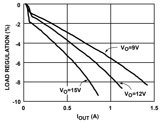
FIGURE 8. V_{\text{BOOST}} LOAD REGULATION AT V_{\text{IN}}=5\text{V} (P MODE)
