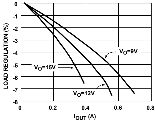
FIGURE 7. V_{\text{BOOST}} LOAD REGULATION AT V_{\text{IN}}=3\text{V} (P MODE)
