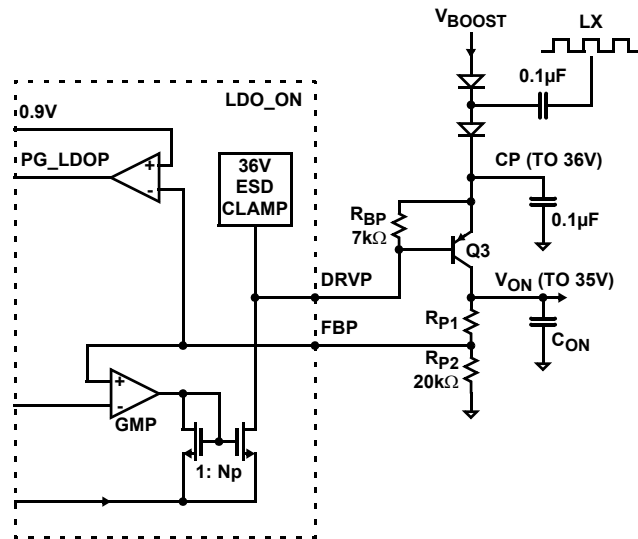
FIGURE 21. V_{\text{ON}} FUNCTIONAL BLOCK DIAGRAM
