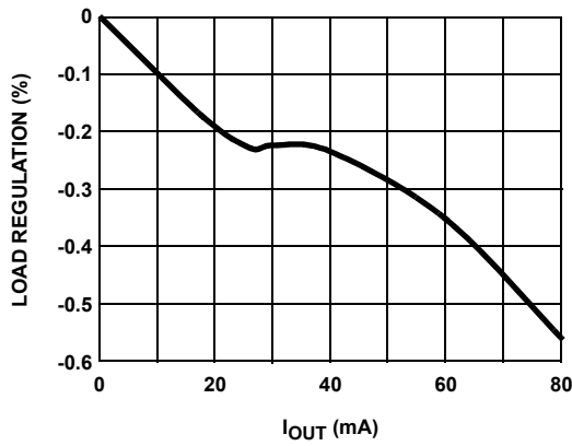
FIGURE 9. V_{\text{ON}} LOAD REGULATION
