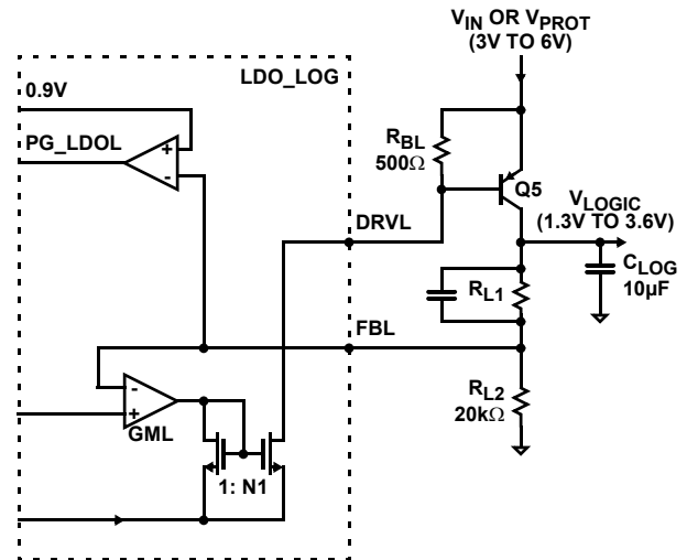
FIGURE 23. V_{\text{LOGIC}} FUNCTIONAL BLOCK DIAGRAM
