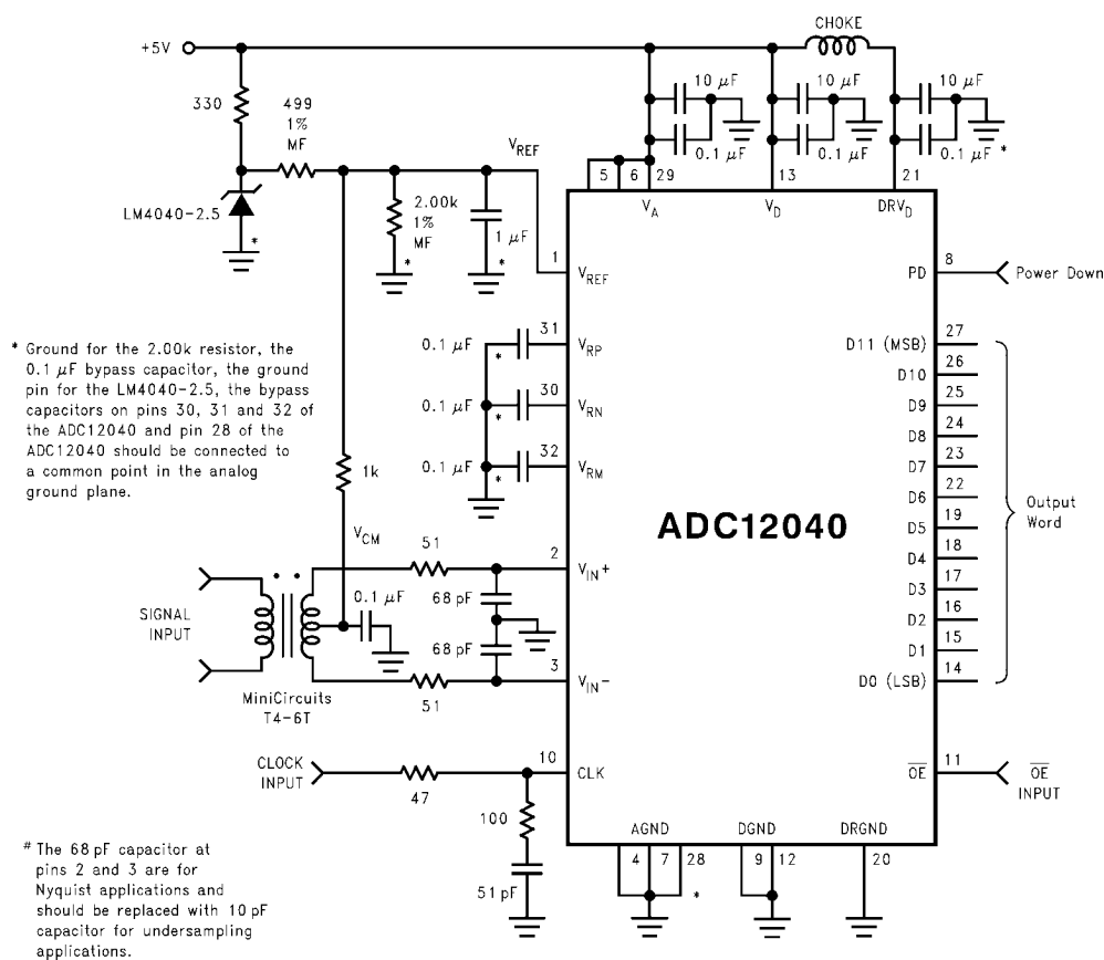
FIGURE 5. Differential Drive Circuit of Figure 4
