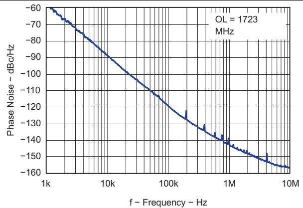
Figure 21. Open Loop VCO Phase Noise
