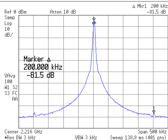
Figure 80. Direct Output: PFD Frequency Spurs
