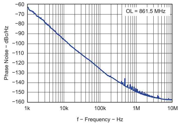
Figure 23. Open Loop VCO Phase Noise
