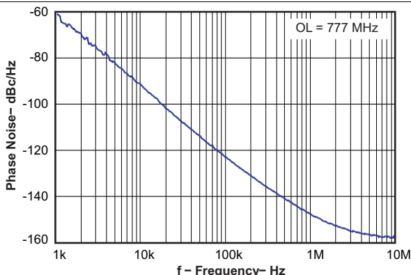
Figure 5. Open Loop VCO Phase Noise
