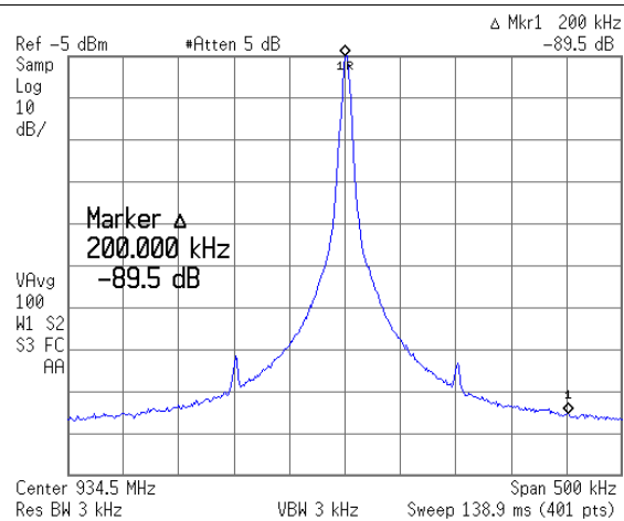
Figure 45. Divide-By-2 Output: PFD Frequency Spurs
