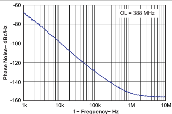
Figure 7. Open Loop VCO Phase Noise
