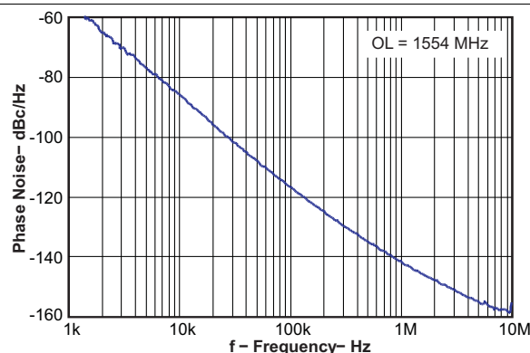
Figure 3. Open Loop VCO Phase Noise
