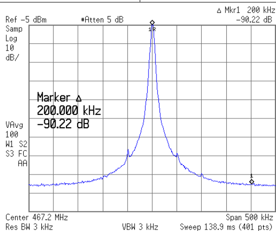
Figure 46. Divide-By-4 Output: PFD Frequency Spurs
