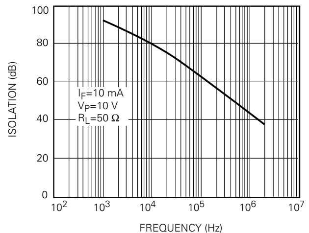
Figure 6. Output Isolation
