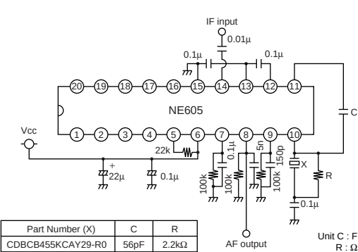
NE605
