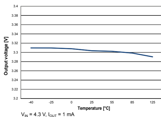
Figure 7. Output voltage vs. temperature ( V_{OUT} = 3.3 \text{ V} , I_{OUT} = 1 \text{ mA} )
