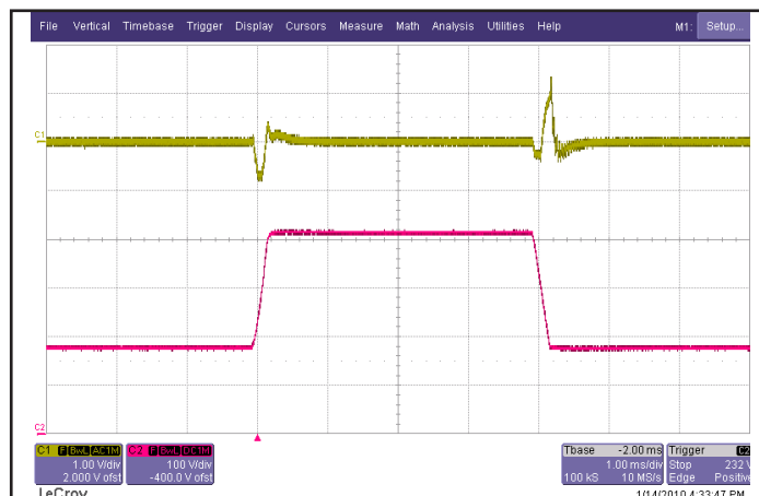
Figure 6: Output voltage response to step-change in input voltage (180V - 425V - 180V), at 6.25A load current. Load cap: 15μF tantalum capacitor and 1uF ceramic cap. Ch 1: V out (1V/div), Ch 2: V in (100V/div).
