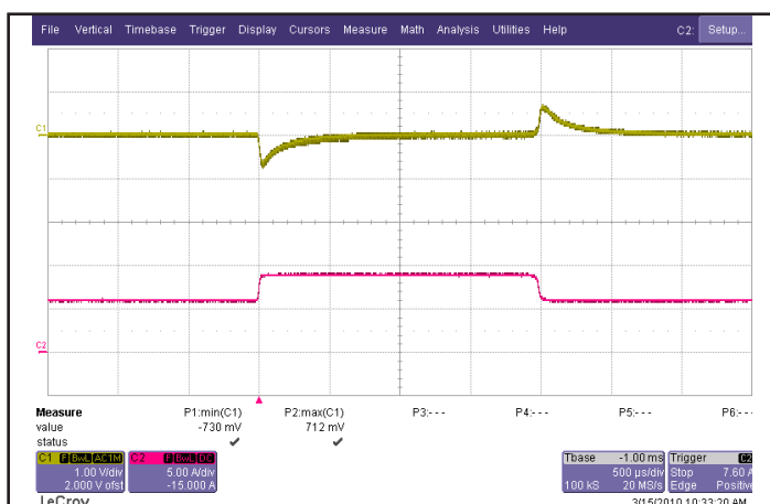
Figure 5: Output voltage response to step-change in load current (50%-75%-50% of I out (max); dI/dt = 0.1A/μs). Load cap: 15μF tantalum cap and 1μF ceramic cap. Ch 1: V out (1V/div), Ch 2: I out (5A/div).
