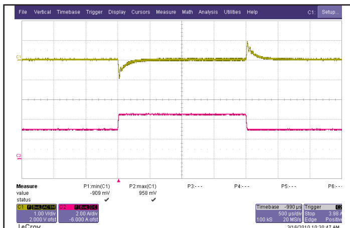
Figure 5: Output voltage response to step-change in load current (50%-75%-50% of I out (max); dI/dt = 0.1A/μs). Load cap: 15μF tantalum cap and 1μF ceramic cap. Ch 1: V out (1V/div), Ch 2: I out (2A/div).
