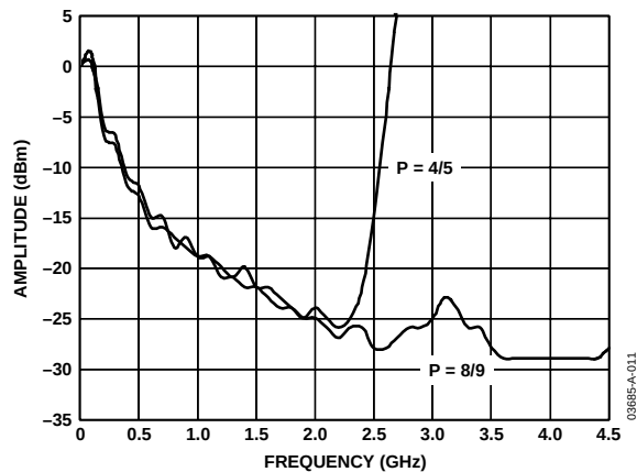
Figure 12. RF Input Sensitivity
