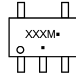
SC-88A (SC-70-5/SOT-353) CASE 419A-02
