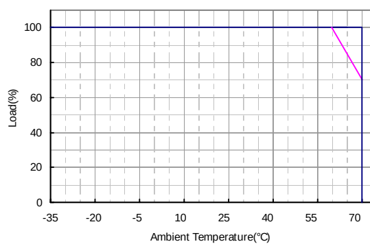
Ambient Temperature vs. Load
