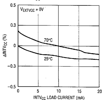
INTV_{CC} Regulation vs INTV_{CC} Load Current
