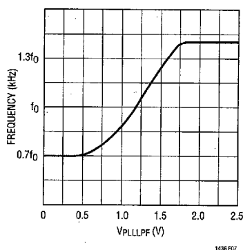
Figure 7. Operating Frequency vs V_{PLLPF}
