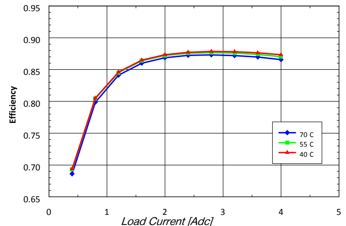
Fig. 12V.6: Efficiency vs. load current and ambient temperature for SQ24T/S04120 converter mounted vertically with V_{in} = 24V and air flowing from pin 3 to pin 1 at a rate of 200 LFM (1.0 m/s).
