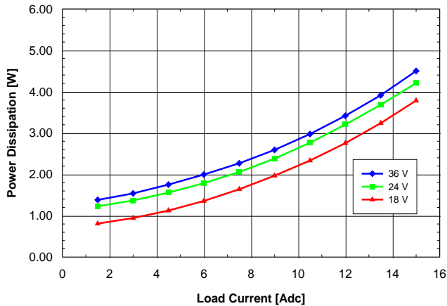
Fig. 1.2V.7: Power dissipation vs. load current and input voltage for SQ24T/S15012 converter mounted vertically with air flowing from pin 3 to pin 1 at a rate of 300 LFM (1.5 m/s) and T_a = 25^\circ\text{C} .
