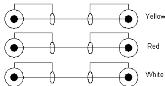
Wiring Diagram
