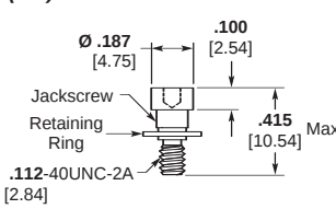
Part Number 6-1532137-0 Jackscrew Assembly Low Profile (N) 096-0002-0065 M83513/5-12 (NM) S96-0002-0091
