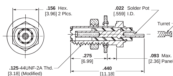
Rear Mount Receptacle w/ Locking Interface 1
