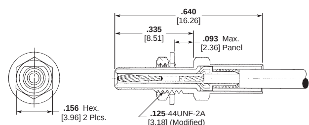
Straight Bulkhead Jack 1 Part Number 141-1001-0001 Instruction Sheet Number 408-08512 Former MICRODOT I.S. Number RF-ASMB-15
