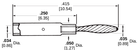
Part Number 096-0526-0000
