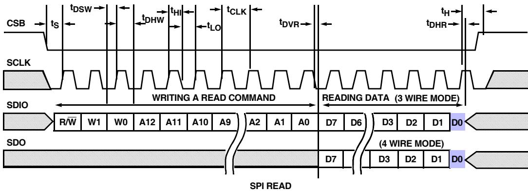
FIGURE 38. SPI READ
