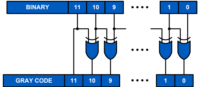
FIGURE 33. BINARY TO GRAY CODE CONVERSION
