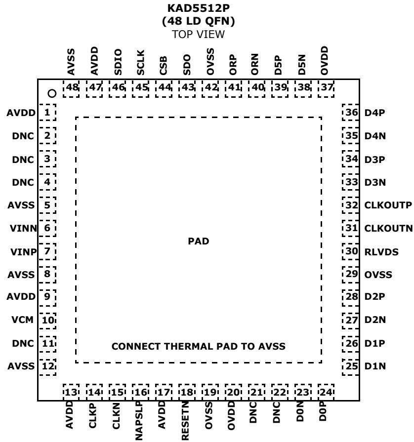
FIGURE 2. PIN CONFIGURATION
