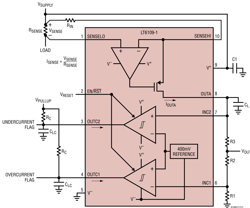
Figure 11. Typical Configuration with Alternative R_{\text{OUT}} Configuration
