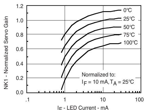
Fig. 9 Normalized Servo Gain vs. LED Current and Temperature
