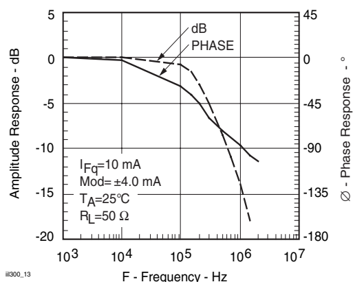
Fig. 13 Amplitude and Phase Response vs. Frequency
