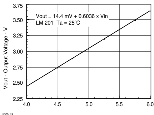
Fig. 19 Transfer Gain
