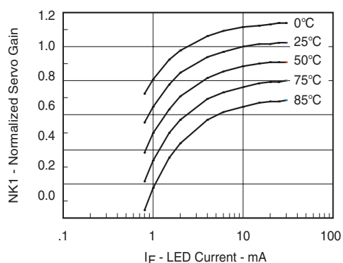
Fig. 8 Servo Gain vs. LED Current and Temperature
