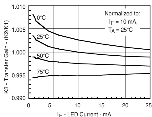
Fig. 11 Normalized Transfer Gain vs. LED Current and Temperature
