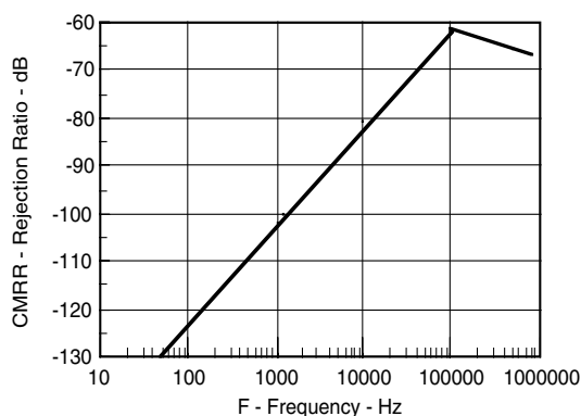
Fig. 14 Common-Mode Rejection
