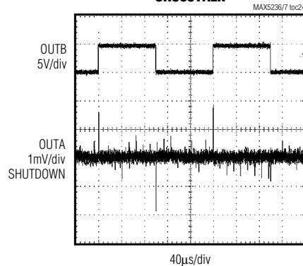
MAX5237 CROSSTALK
