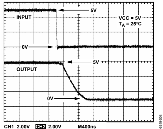
Figure 11. Transient Response—Falling
