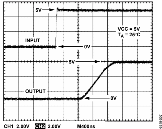
Figure 10. Transient Response—Rising
