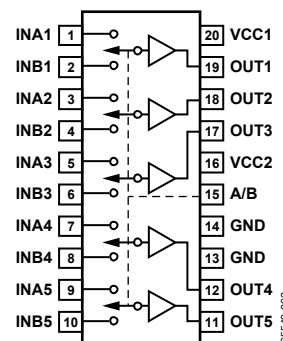
Figure 2. ADD8505, 5-Channel Buffer
