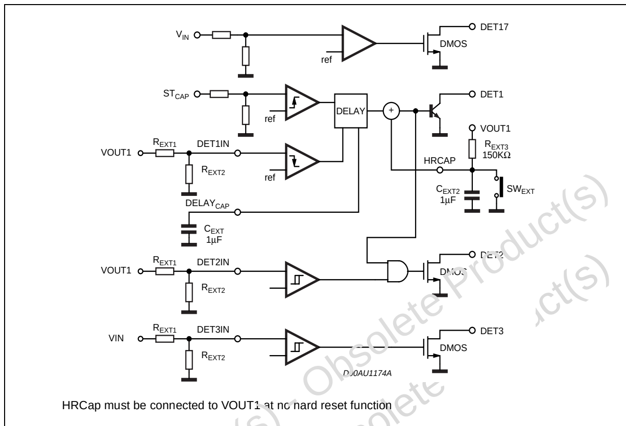
Figure 2. Reset Function
