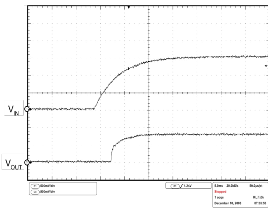
Figure 16. Start-up transient
