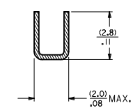
SECTION C-C
