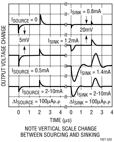
Load Transient Response LT1021-10, C LOAD = 1000pF
