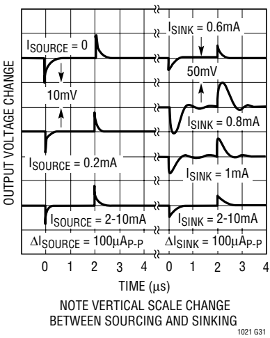
Load Transient Response LT1021-10, C LOAD = 0
