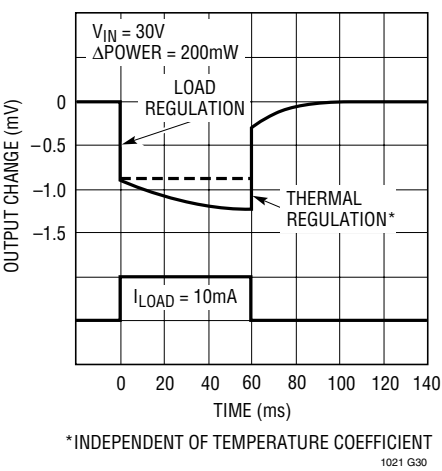
Thermal Regulation LT1021-10
