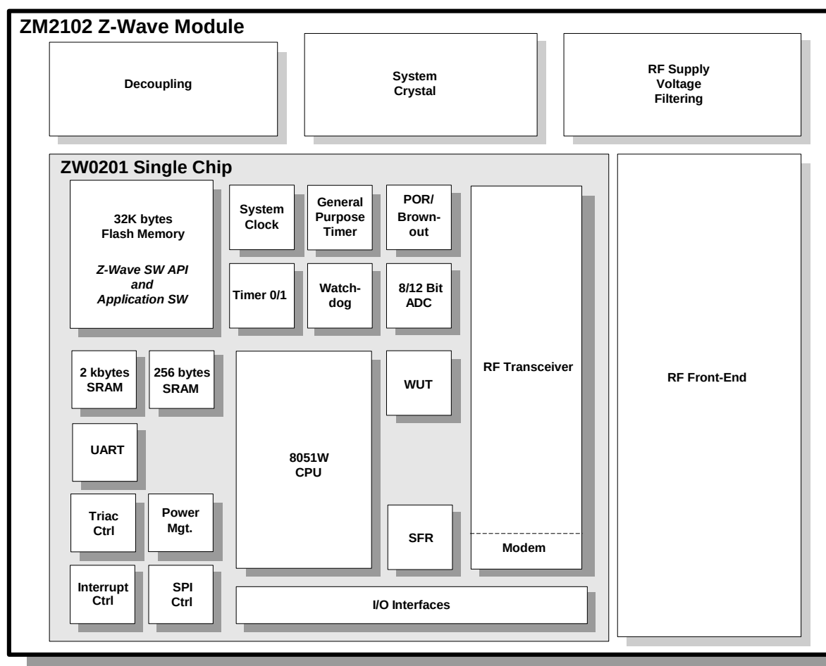
Figure 1 ZM2102 Z-Wave Module Block Diagram
