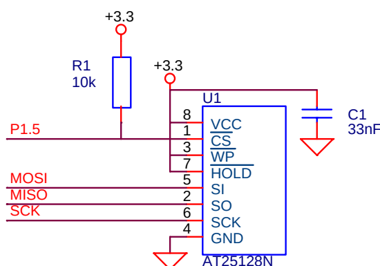
Figure 8 External EEPROM
