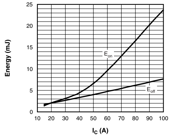
Fig. 9 - Typical IGBT Energy Loss vs. I_c T_J = 125 °C, L = 500 \mu H, V_{CC} = 600 V, R_g = 5 \Omega , V_{GE} = 15 V
