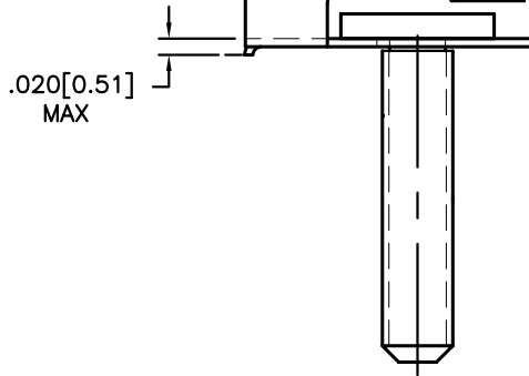
AUX. VIEW "A" TERMINAL w/o TAIL
