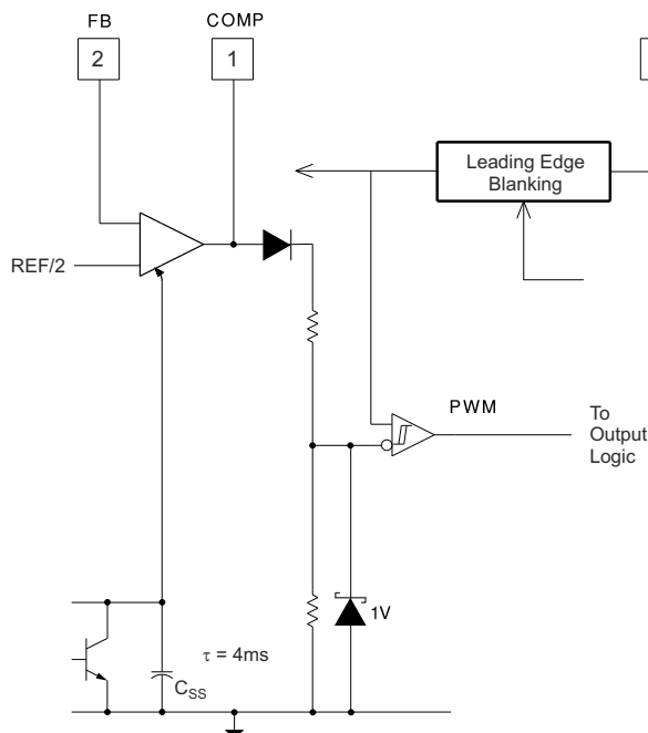
Figure 7-20. Detailed Block Diagram for Soft-Start
