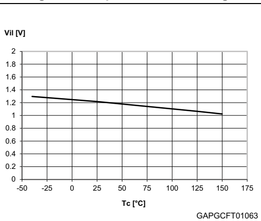
Figure 20. Input low level voltage
