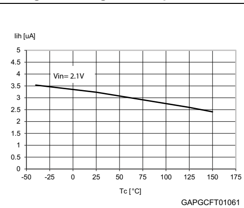
Figure 18. High level input current
