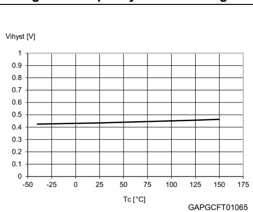
Figure 22. Input hysteresis voltage
