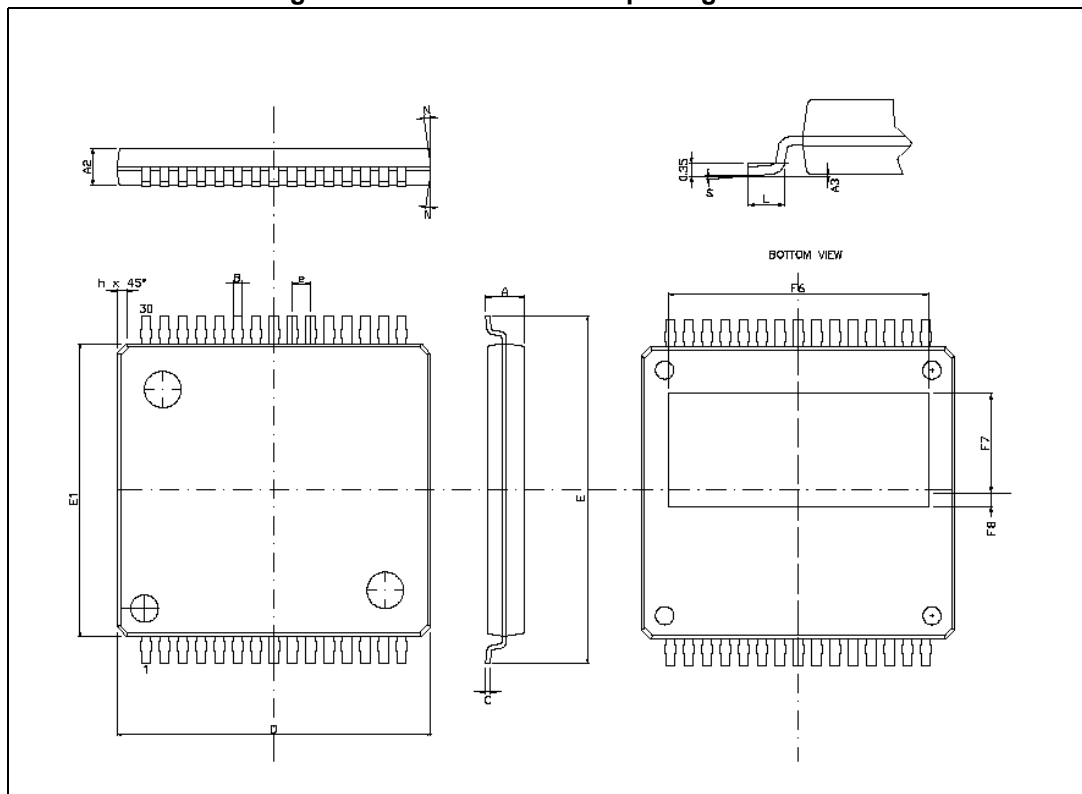
Figure 43. MultiPowerSO-30 package outline
