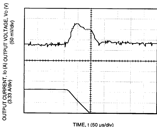
Figure 6. Typical FE150N Transient Response to Step Decrease in Load from 50% to 25% of Full Load at Room Temperature and 48 V Input (Waveform Averaged to Eliminate Ripple Component.)
