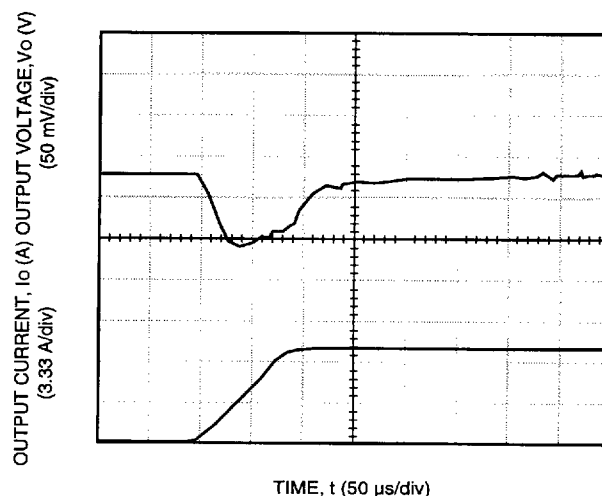
Figure 7. Typical FE150N Transient Response to Step Increase in Load from 50% to 75% of Full Load at Room Temperature and 48 V Input (Waveform Averaged to Eliminate Ripple Component.)
