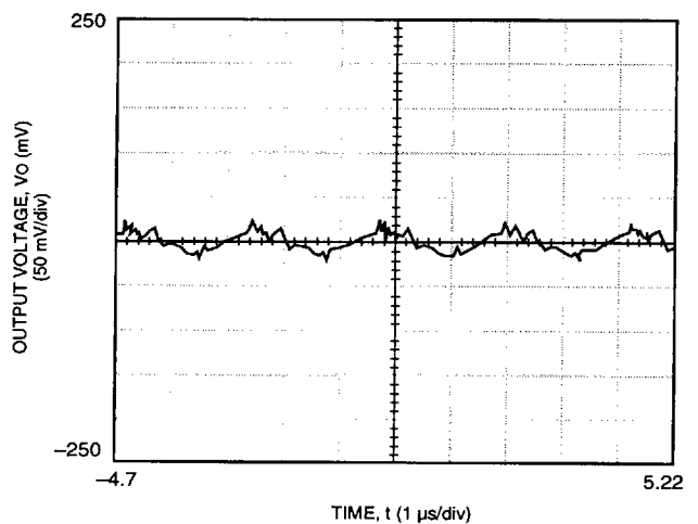
Figure 5. Typical FE150N Output Ripple Voltage at Room Temperature, 48 V Input, and 28.8 A Output
