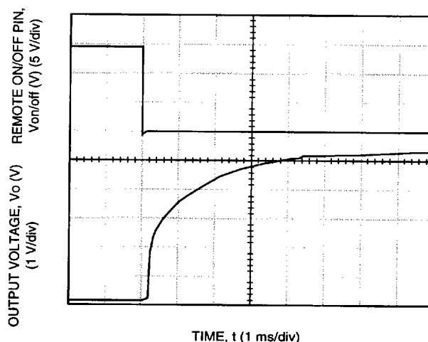
Figure 8. Typical FE150N Start-Up Transient at Room Temperature, 48 V Input, and 12.5 A Output
