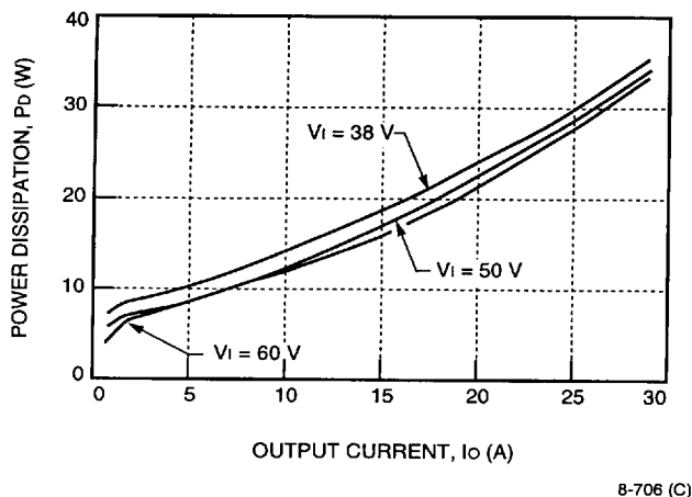
Figure 22. FE150N Power Dissipation as Heat vs. Output Current
