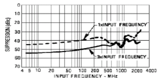
Harmonic Suppression vs. Input Frequency
