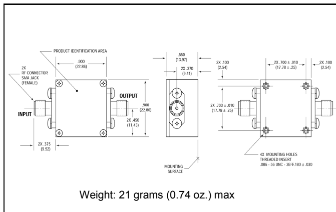
Outline Drawing: SMA Connectorized *
