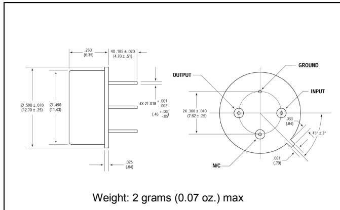
Outline Drawing: TO-8 *
