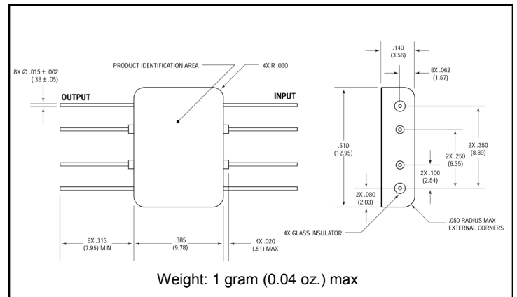
Outline Drawing: Flatpack *
