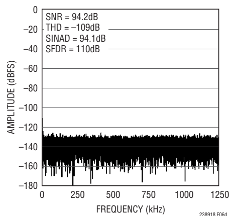
Figure 6d. 32k Point FFT f_{\text{SMPL}} = 2.5\text{Mpsps} , f_{\text{IN}} = 2\text{kHz} , for Circuit Shown in Figure 6a; Driven with Bipolar Inputs
