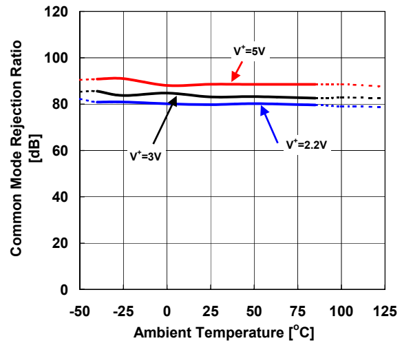
Common Mode Rejection Ratio2 vs. Ambient Temperature
