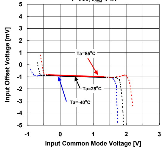
Input Offset Voltage vs. Input Common Mode Voltage (Ambient Temperature) V^+=2.2\text{V} , V_{\text{COM}}=V^+/2\text{V}
