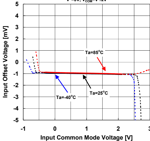
Input Offset Voltage vs. Input Common Mode Voltage (Ambient Temperature) V^+=3\text{V} , V_{\text{COM}}=V^+/2\text{V}
