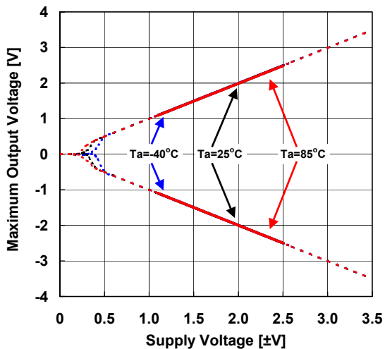
Maximum Output Voltage vs. Supply Voltage (Ambient Temperature)
