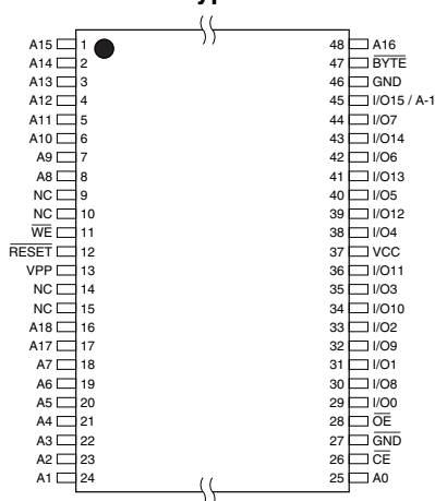
AT49BV8192A(T) TSOP Top View Type 1
