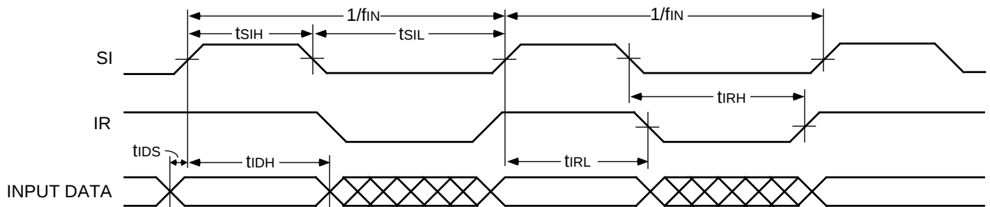
Figure 2. Input Timing
