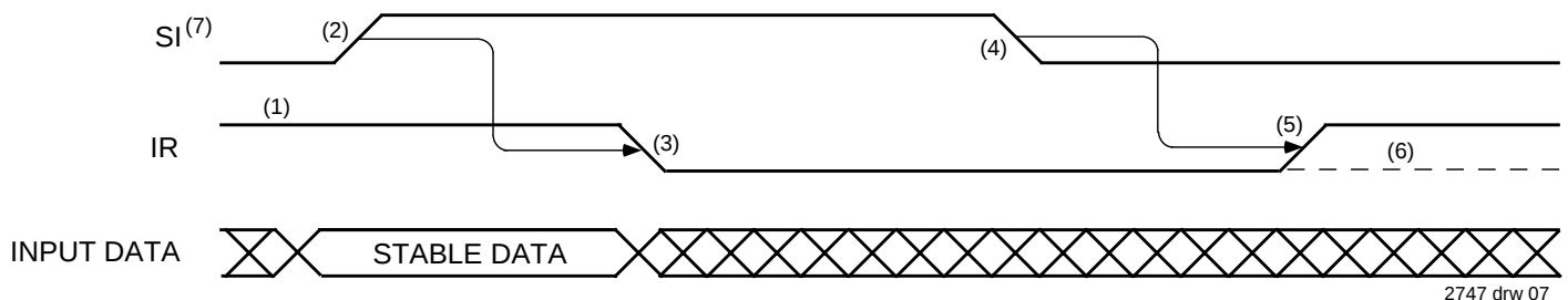
Figure 2. Input Timing
