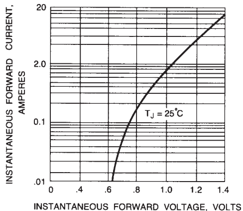
Fig. 1 - TYPICAL FORWARD CHARACTERISTICS
