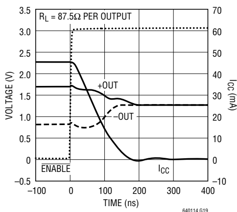
Turn-Off Time
