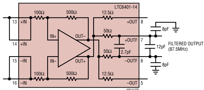
Figure 5. LTC6401-14 Internal Filter Topology Modified for Low Filter Bandwidth (Three External Capacitors)
