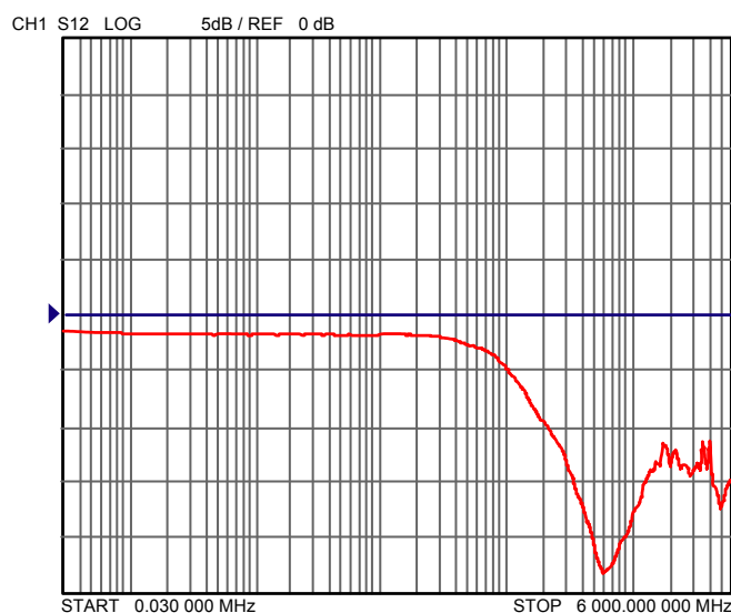
Figure 6 – Frequency response curve. Low insertion loss in the pass band and -20dB attenuation at 800-900 MHz. Better than -10dB attenuation at the WLAN frequencies of 2.4 and 5.0-6.0 GHz.
