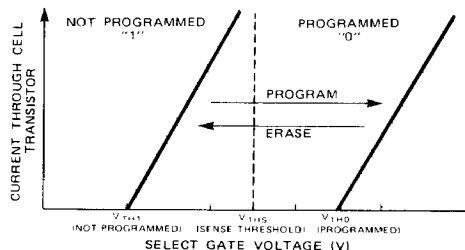
Fig. 2 — Memory Cell Threshold Shift
