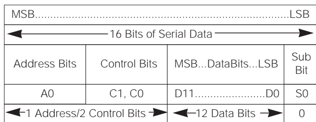
Figure 4. Serial-Data Format
