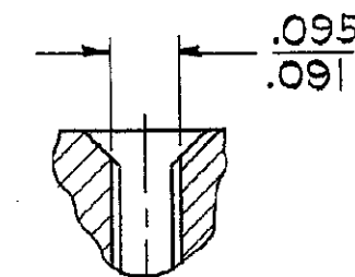
SECT. B-B
