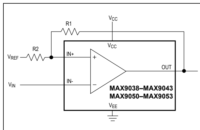
Figure 1. Additional Hysteresis
